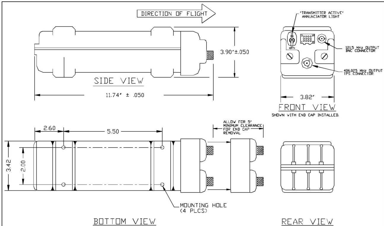
ELT OUTLINE DRAWING
